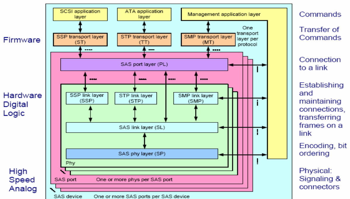
Figure 1; Serial Attached SCSI Multi-protocol Connection Support
